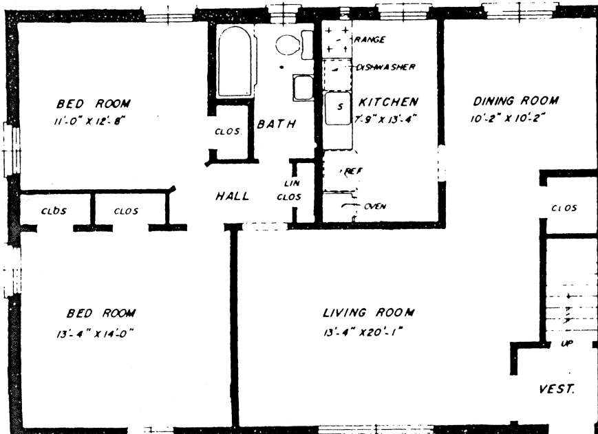
FIRST FLOOR PLAN 5 ROOM APT.
